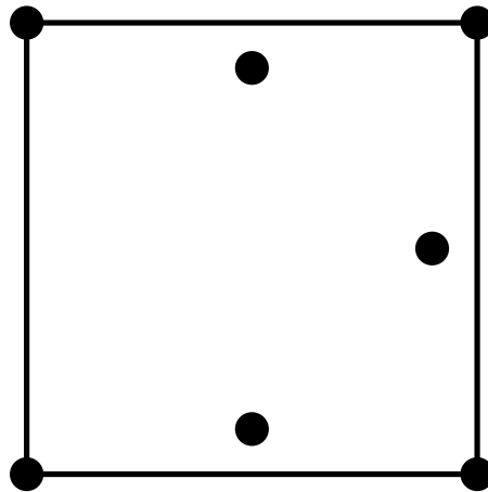
Sample Input 2
