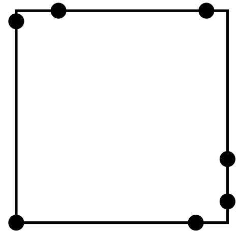
Sample Input 3
