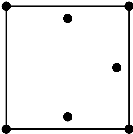
Sample Input 1
